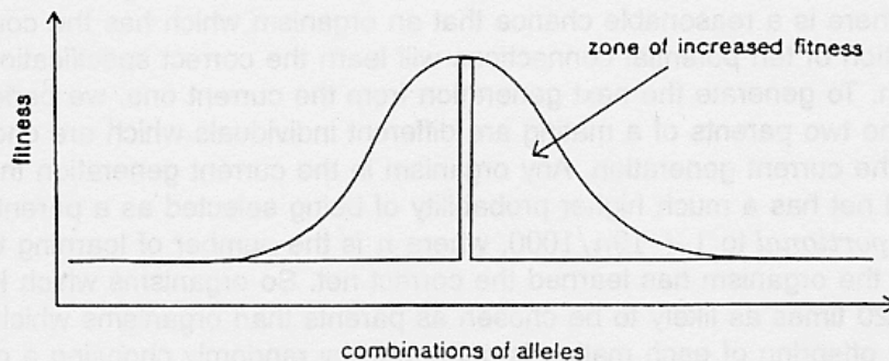
FIGURE 1 The shape of the search space in which evolution operates. The horizontal axis represents combinations of alleles and so it is not really one-dimensional. Without learning, the search space has a single spike of high fitness. One cannot do better than random search in such a space. With learning, there is a zone of increased fitness around the spike. This zone corresponds to genotypes which allow the correct combination of potential connections to be learned.
